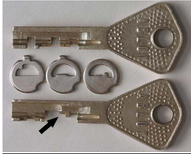
Two different keyshape profiles used in ONE Master key system
