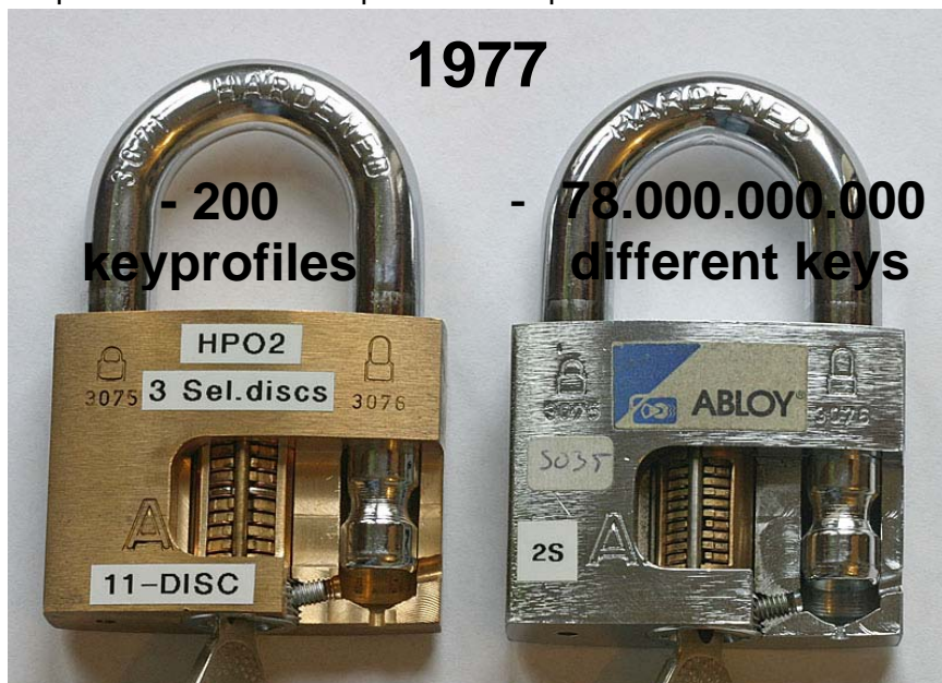
Two High security padlocks from the 70's.
